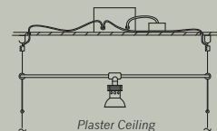
Plaster Ceiling
