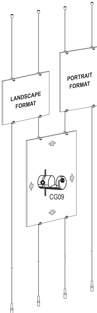
Ceiling/Floor Cable (CA4)
