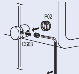
Showcase Fixing
